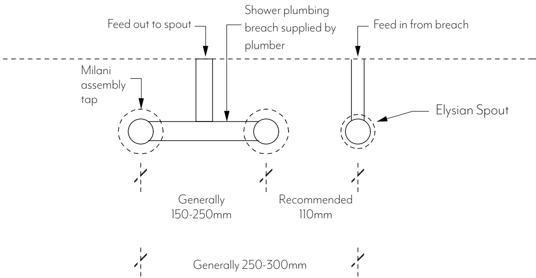
EXAMPLE ONE Offset basin mixer/bath spout setup
